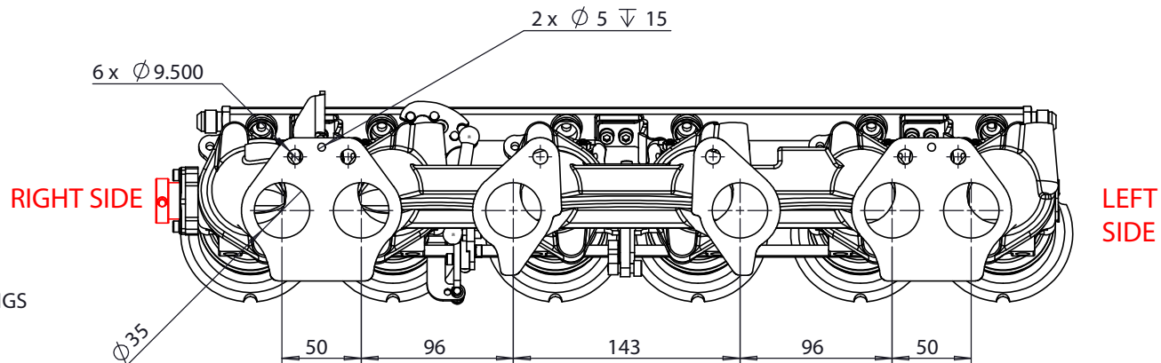
VIEW ON MATING CYLINDER HEAD FACE
