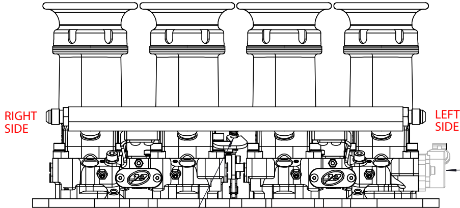
CENTRE PULL CABLE LINKAGE AND IDLE ADJUSTMENT
